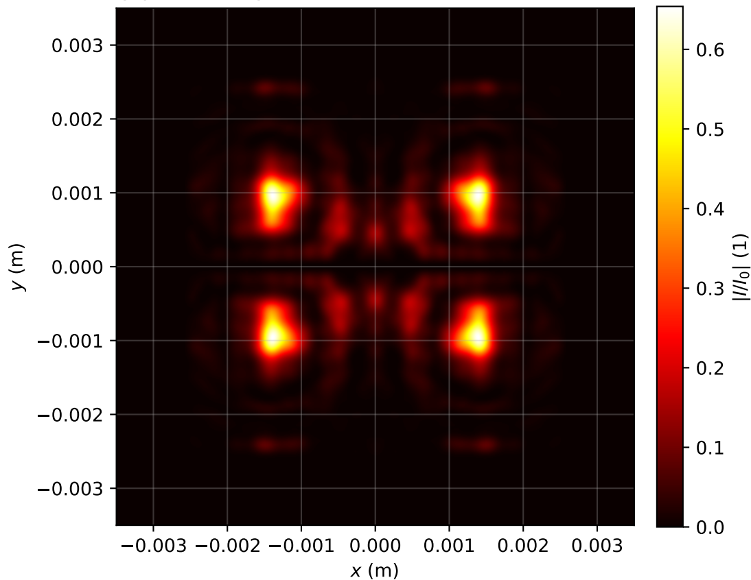
Intensity profile I(x, y, z = 3.582)/I_0 , P_{in}=7.0P_{cr} , artificial time
